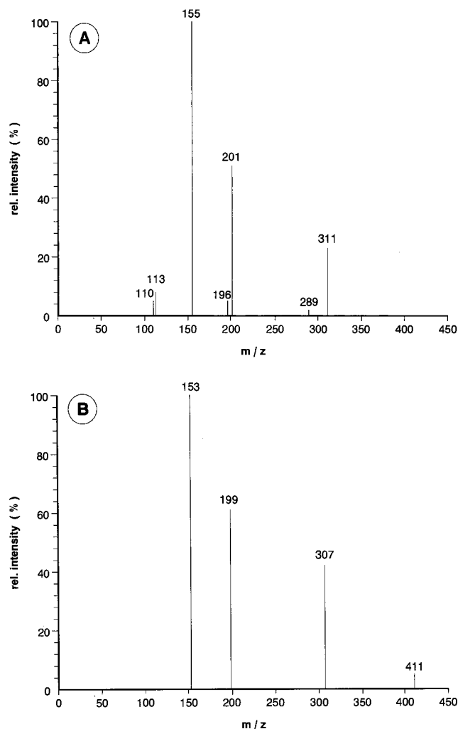
Figure 6. Mass spectra obtained by negative ESI of the labeled (A) and the unlabeled patulin (B).
