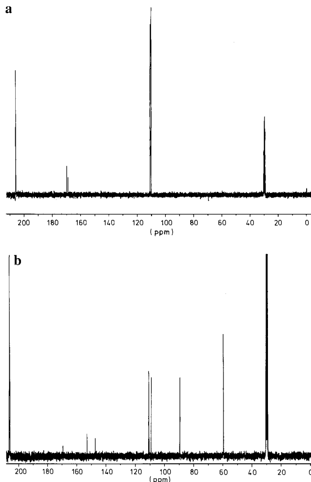
Figure 3. ^{13}\text{C} NMR spectrum of labeled (A) and unlabeled (B) patulin. Signals at 29.9 and 206.3 ppm are caused by the solvent acetone- d_6 .
