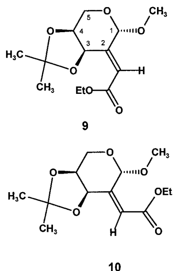
Figure 2. Structure of geometric isomers 9/10 formed by reaction of ketone 4 with unlabeled ethyl bromoacetate.
