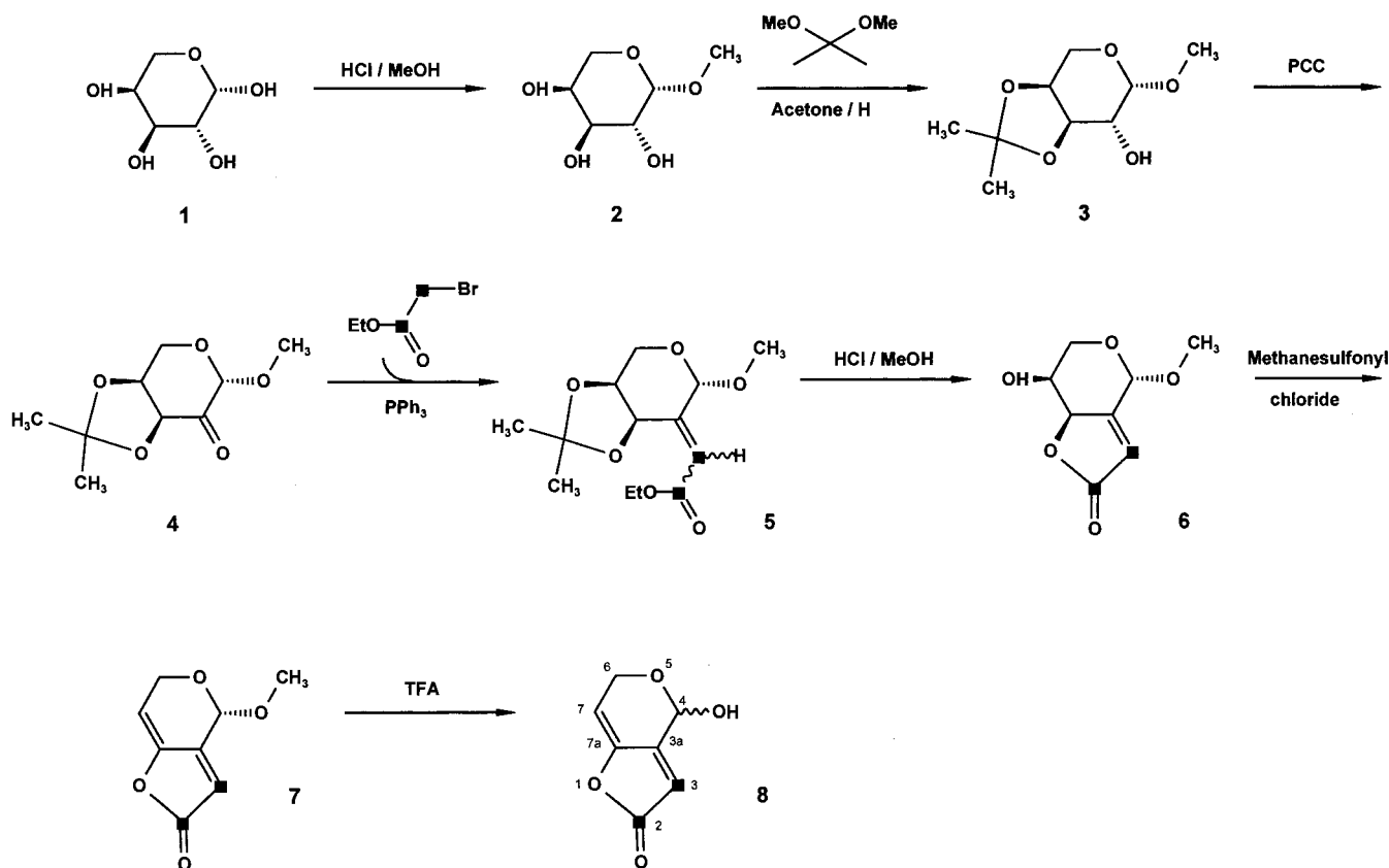
Figure 1. Synthetic route used in the preparation of [ ^{13}\text{C} ] _2 -patulin.
