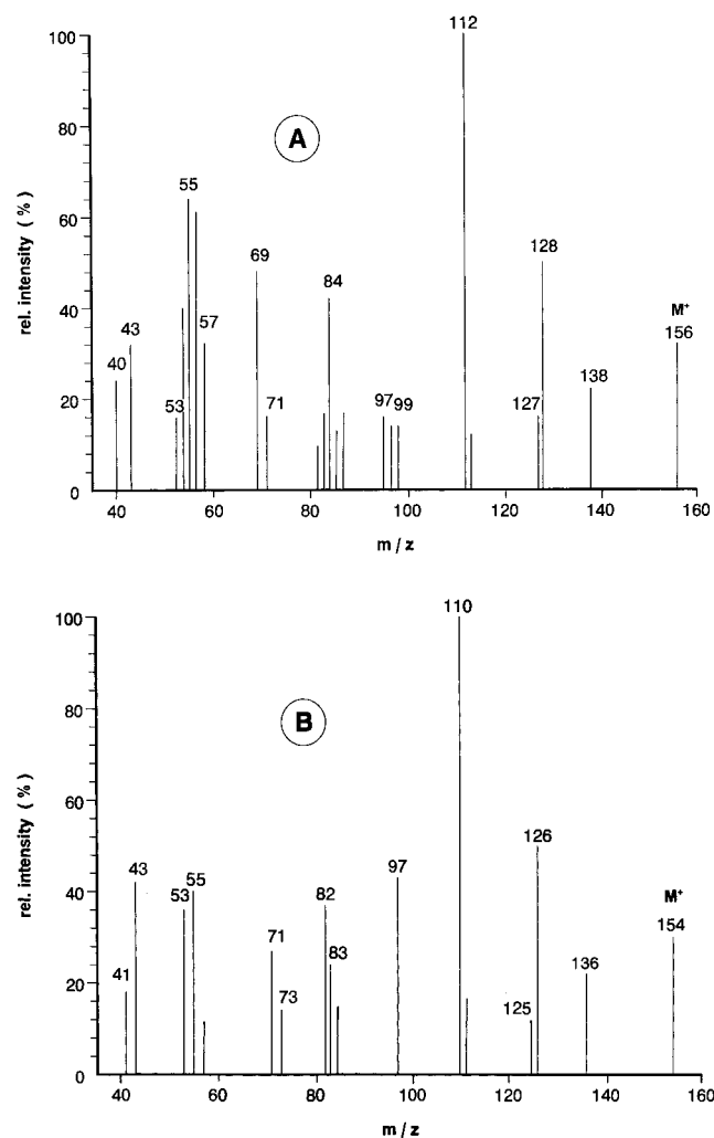
Figure 4. Mass spectrum of labeled (A) and unlabeled patulin (B) obtained by mass spectrometry in the electron impact mode using the direct insertion technique.
