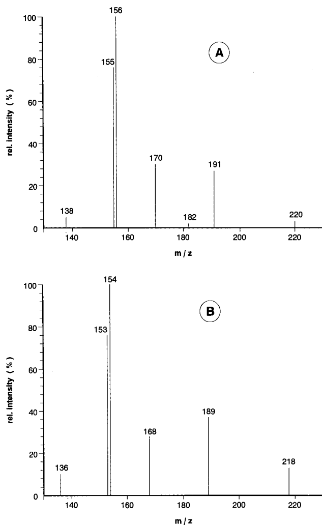
Figure 8. Mass spectra obtained by APCI of the labeled (A) and the unlabeled patulin (B).
