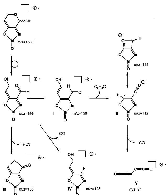
Figure 5. Fragmentation of the labeled patulin during electron impact ionization.
