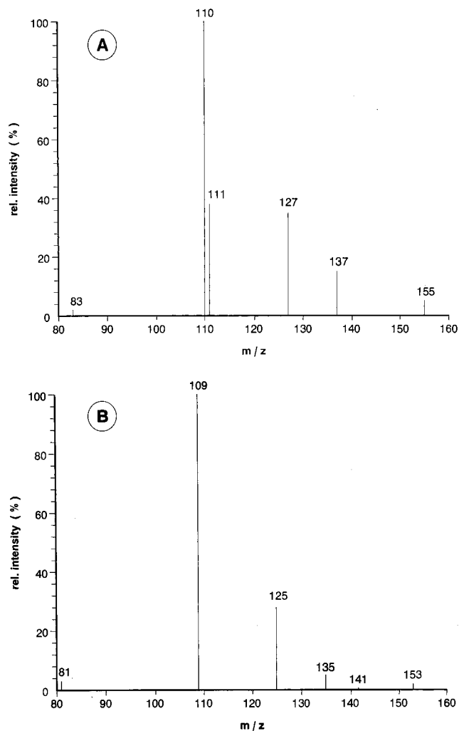
Figure 7. Mass spectra obtained by CID of the molecular ions m/z 156 (labeled patulin; A) and m/z 154 (unlabeled patulin; B).
